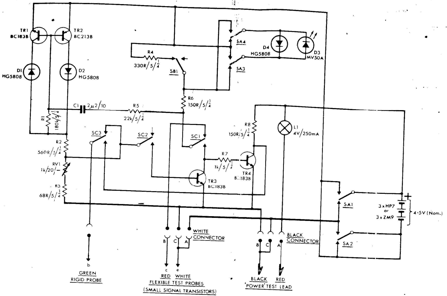
Circuit Diagram for Avo Transistor Tester
